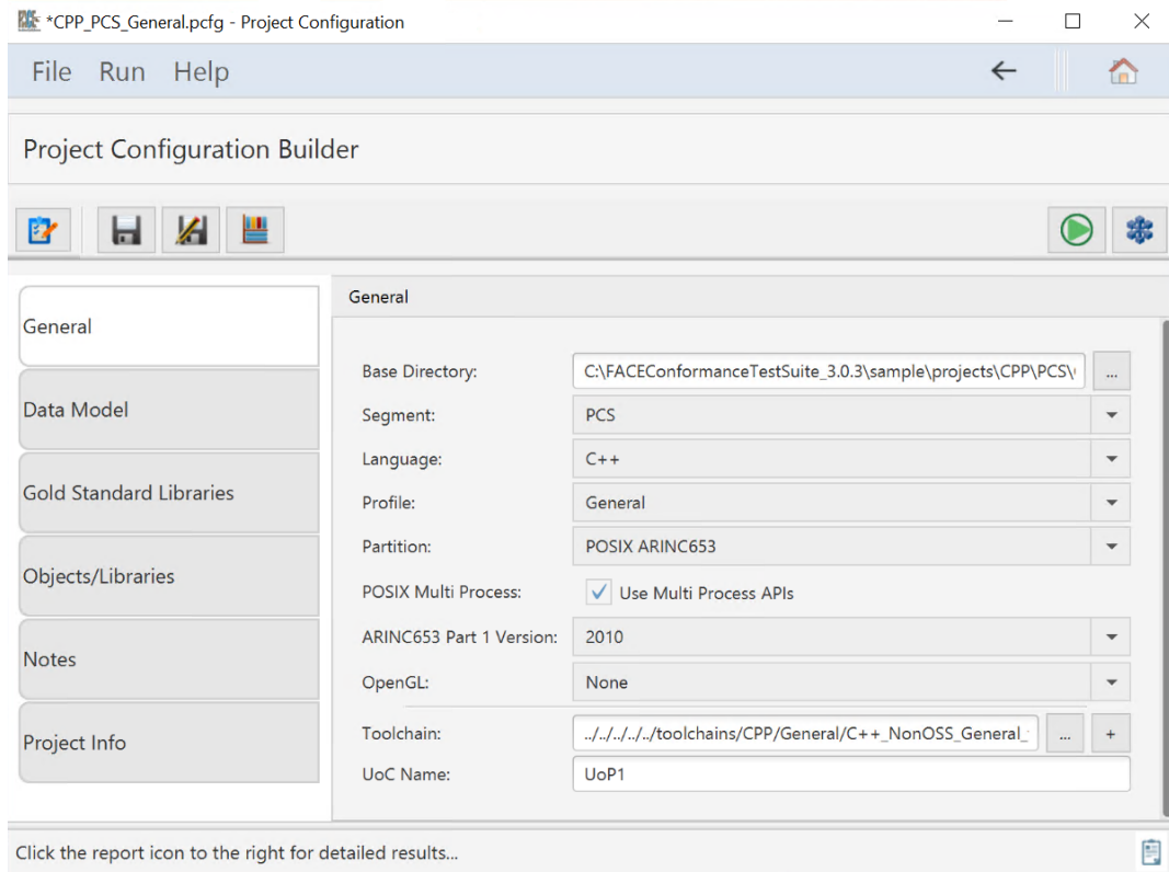
Figure 91. Select PCS in the General Tab of the Project Configuration Builder
