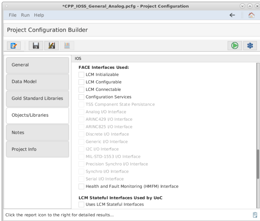
Figure 78. FACE Interfaces Used
