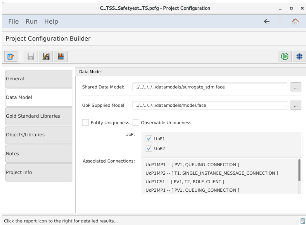
Figure 63. Data Model tab
