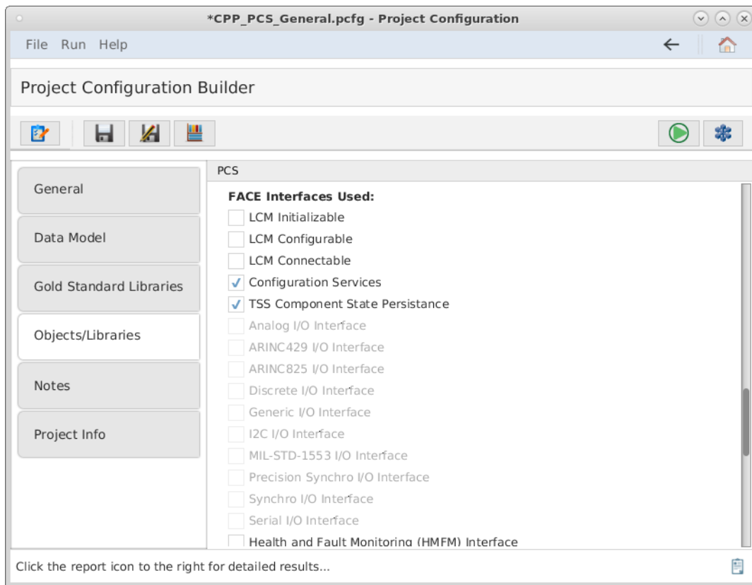
Figure 45. FACE Interfaces Used
