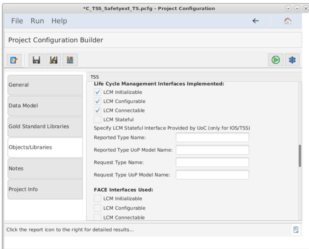
Figure 66. Life Cycle Management
