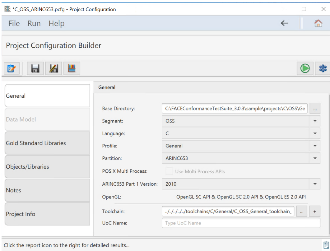
Figure 84. Project Configuration General tab
