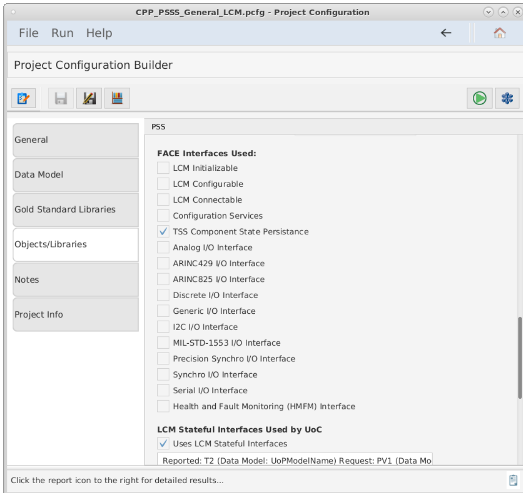
Figure 56. FACE Interfaces Used
