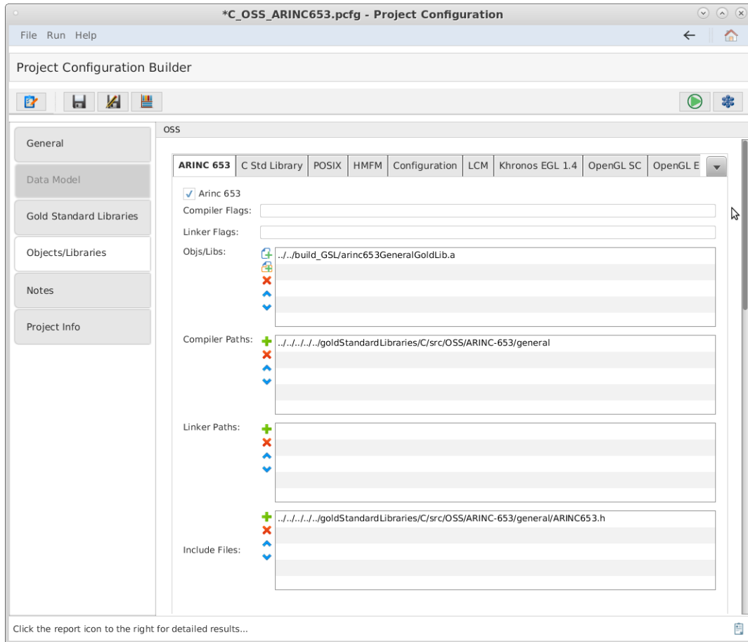
Figure 86. The Project Configuration Builder with the Objects/Libraries tab selected.
