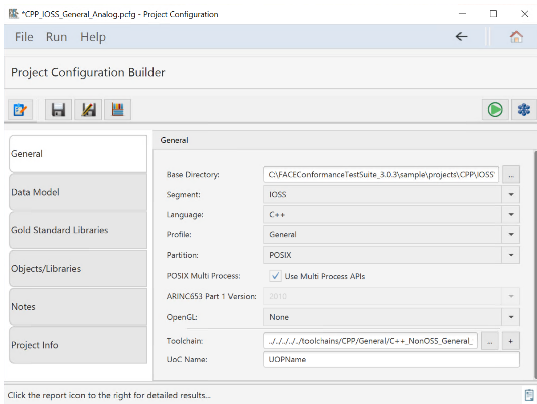
Figure 73. Project Configuration Builder General tab
