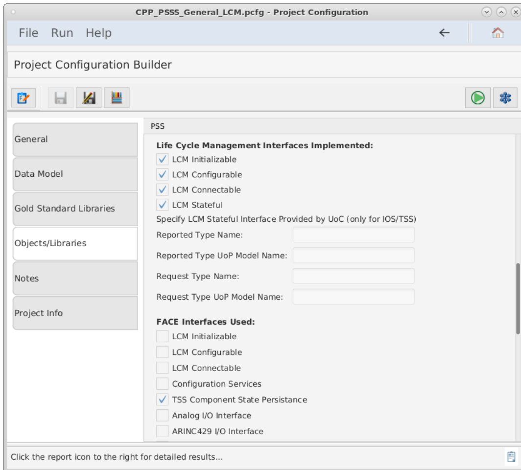
Figure 55. Life Cycle Management
