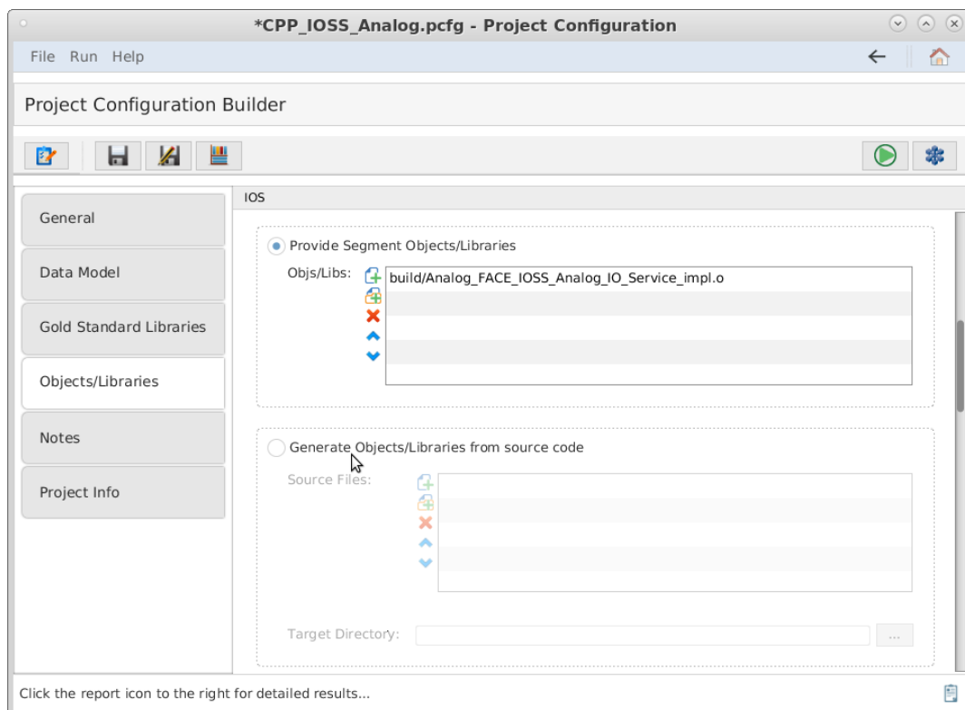
Figure 70. The Project Configuration Builder, with the Objects/Libraries tab selected.
