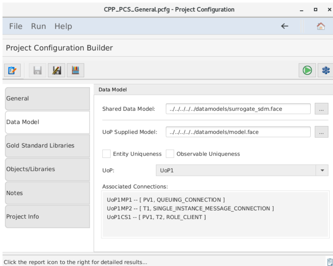
Figure 41. Data Model tab
