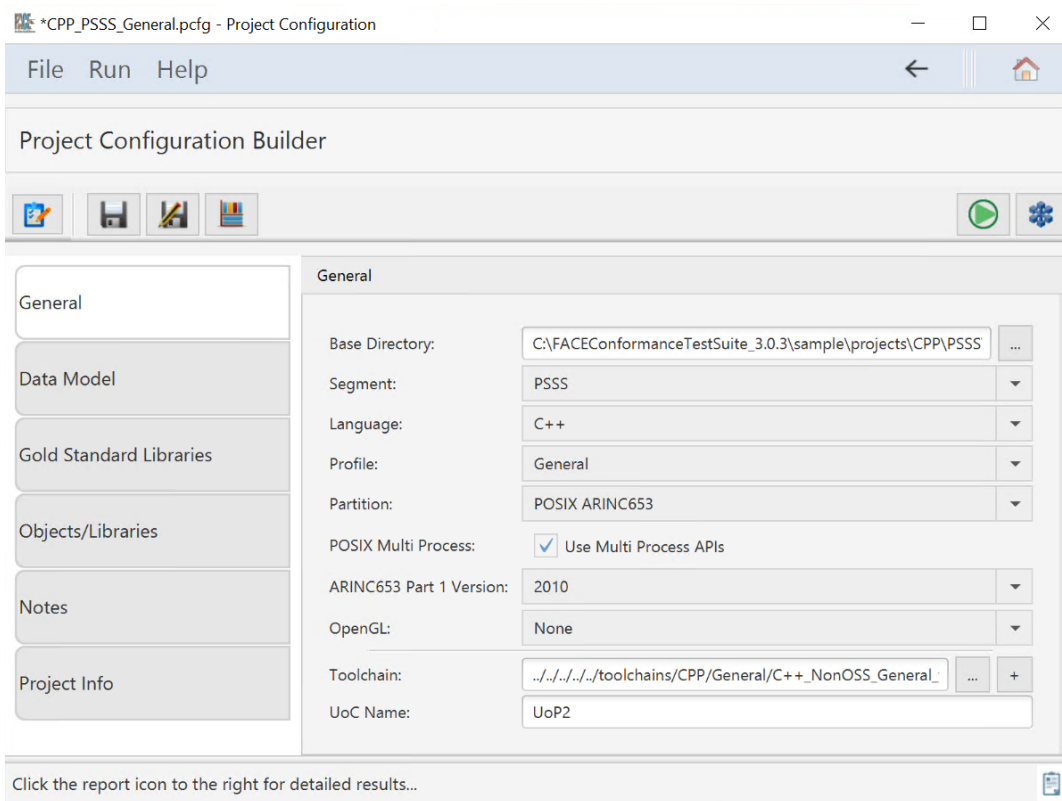
Figure 51. Project Configuration Builder General tab
