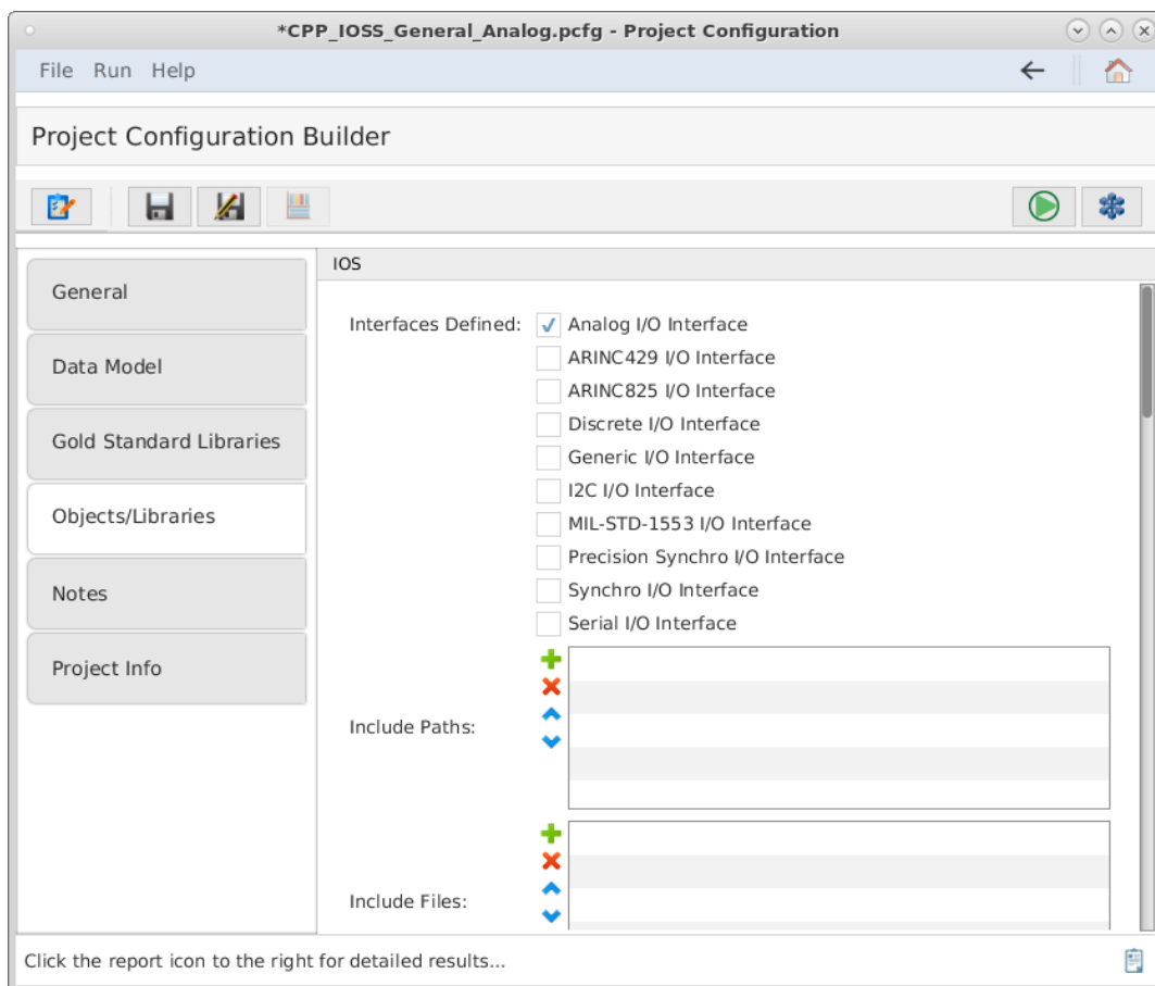
Figure 76. Include Paths and Files
