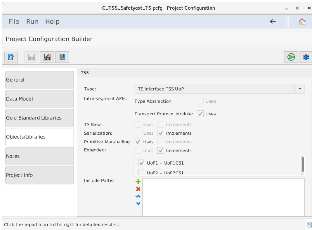
Figure 65. Include Paths and Files
