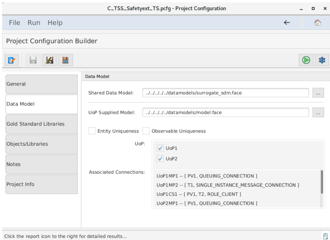
Figure 92. Projection Configuration Builder Data Model tab
