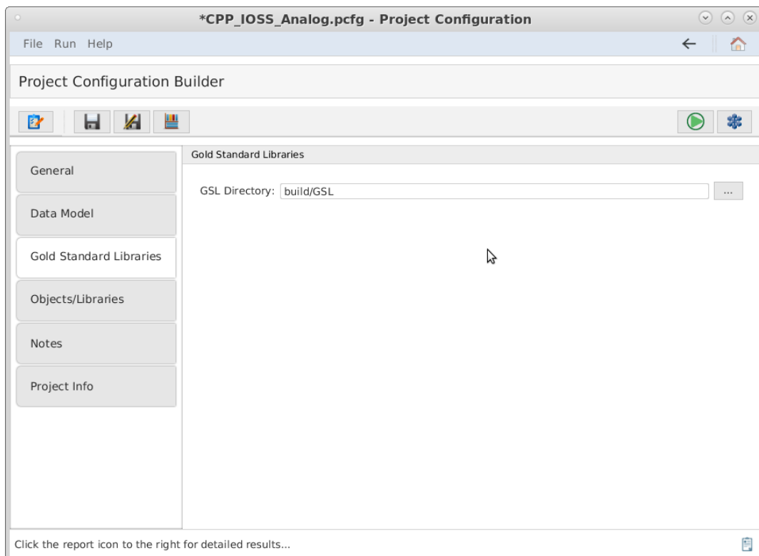
Figure 75. Gold Standard Libraries tab
