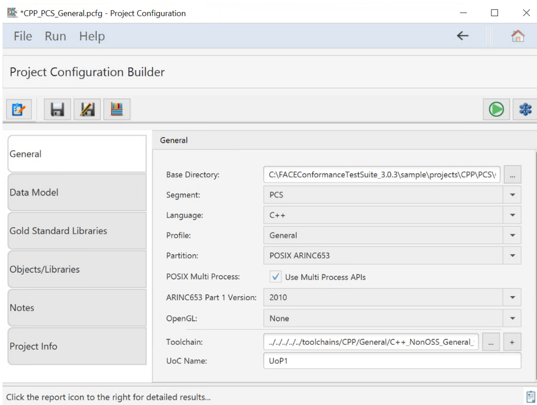
Figure 40. Project Configuration Builder General tab
