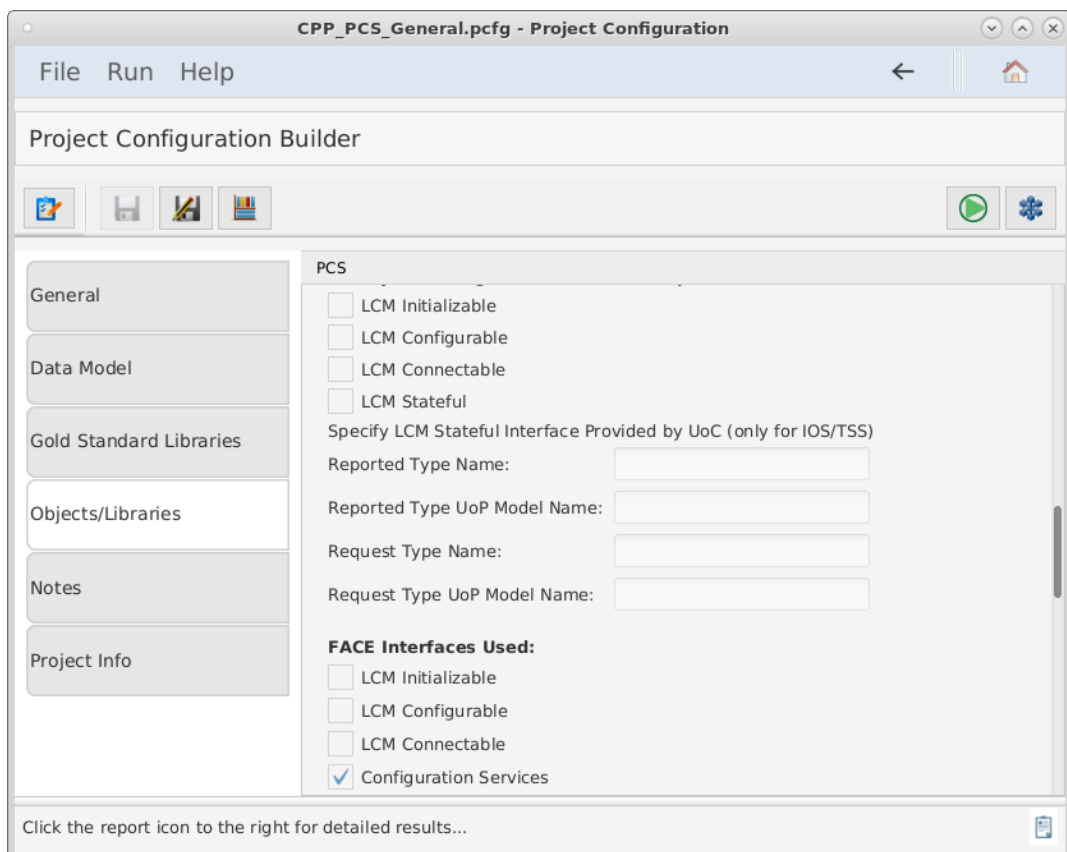
Figure 44. Life Cycle Management
