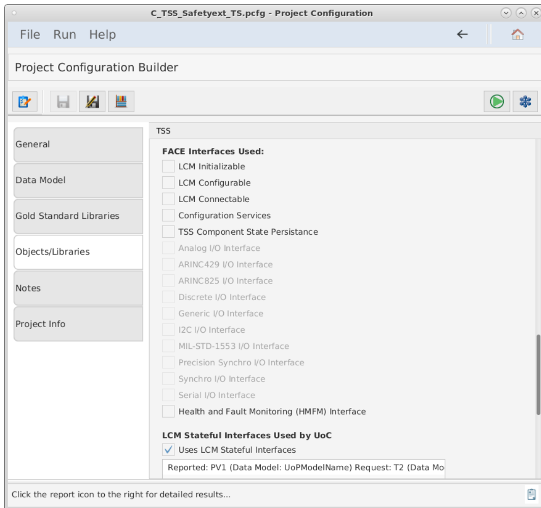
Figure 67. FACE Interfaces Used
