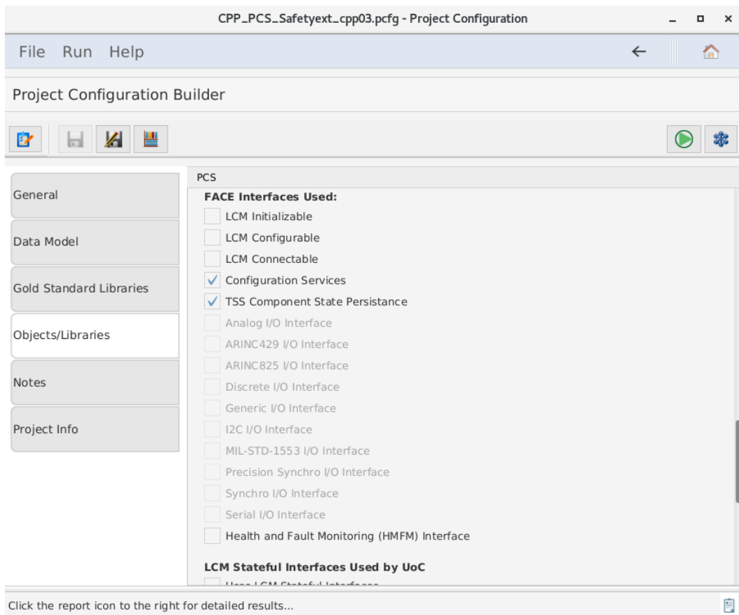
Figure 45. FACE Interfaces Used
