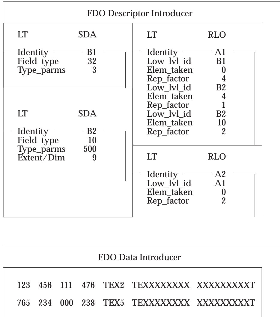
Figure 3-6 Regular Array, Several Field Types
