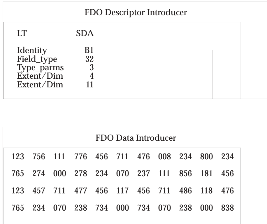
Figure 3-5 Regular Array of Three-Digit Numeric Fields
