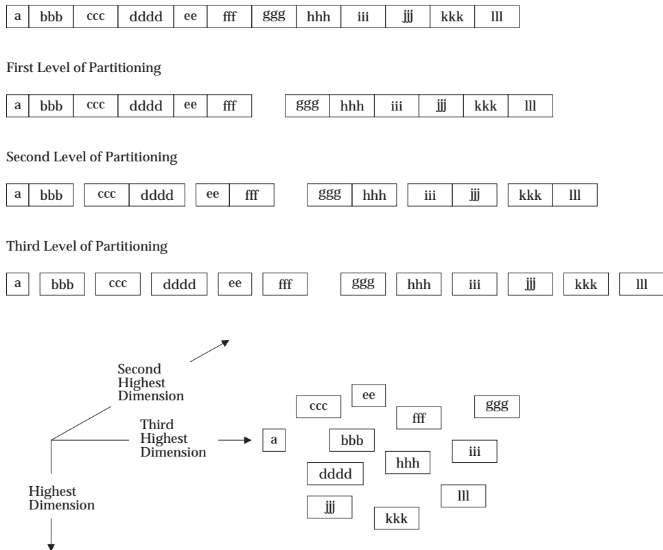
Figure 3-4 Partitioning a Linear String of Fields into Three Dimensions
