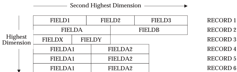
Figure 3-3 General Array Example
