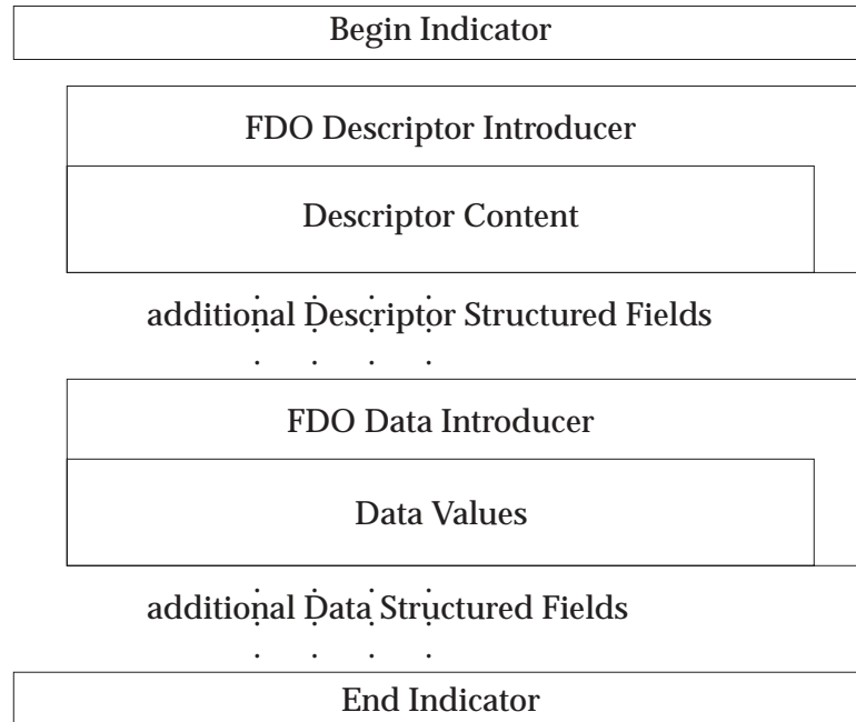
Figure 3-1 Formatted Data Object
