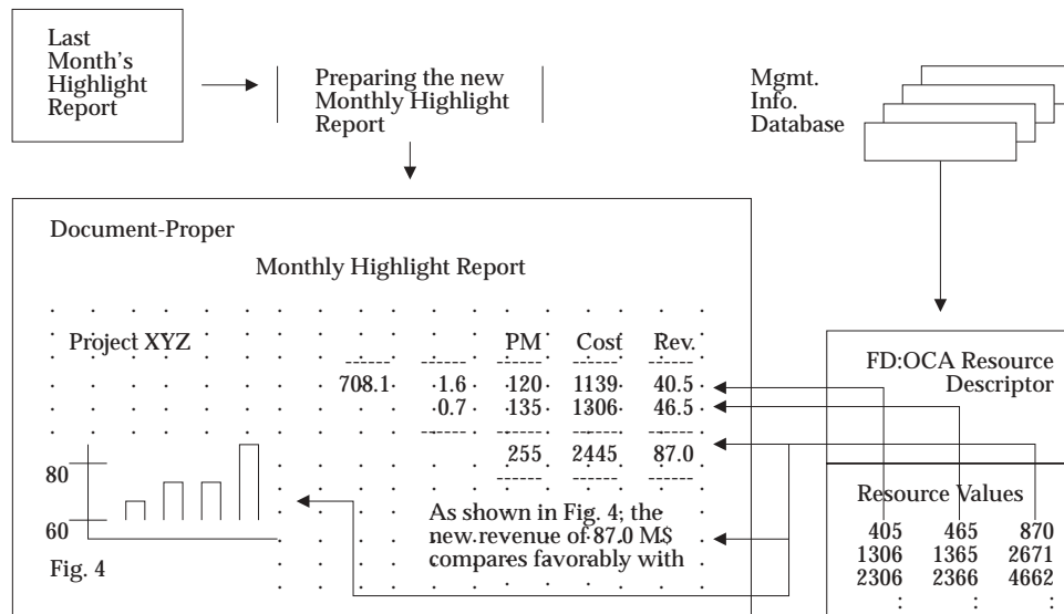
Figure 2-1 Typical FD:OCA Example
