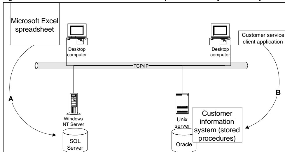
Figure 1. Two-tier Client/Server Architecture Can Be Implemented in Many Different Ways
