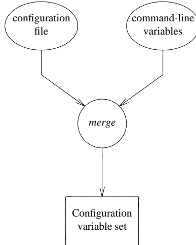
Figure 14. Configuration variable processing in TETware-Lite
