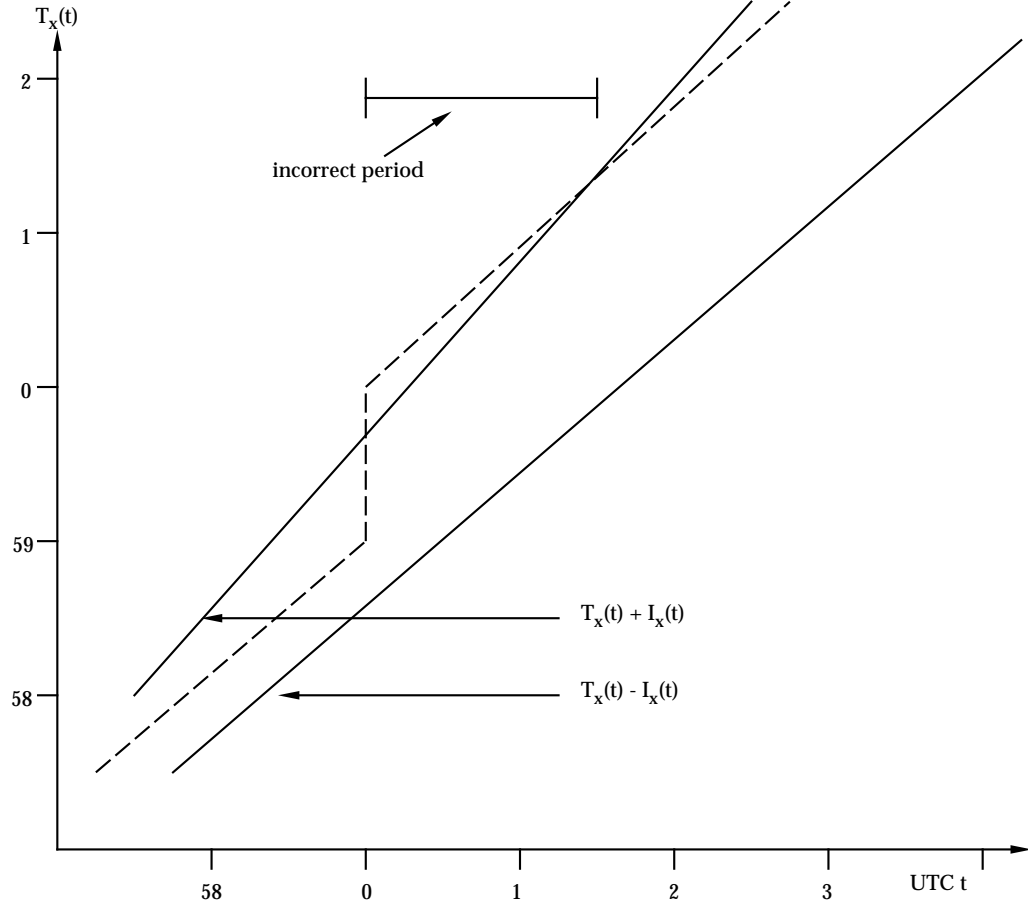
Figure 2-4 How a Negative Leap Second Causes a Clock to Be Incorrect
