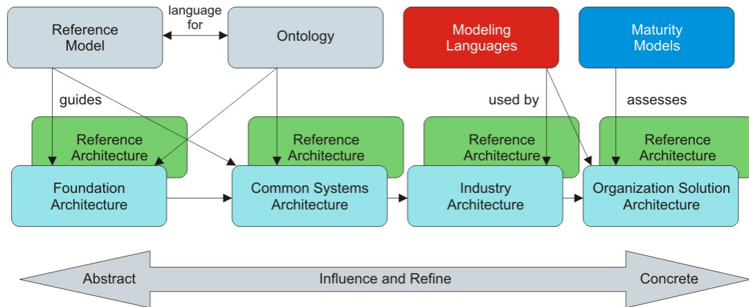
Figure 3: Influence of Reference Model and Ontology on Architecture Work
